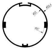
Item No.: GL1080 W: 0.77kg/m T: 1.25mm OD: \Phi 55.4mm ID: \Phi 53mm
