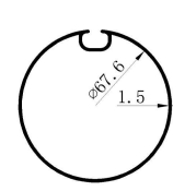
Item No.: GL1076 W: 0.866kg/m T: 1.5mm OD: \Phi 70.6mm ID: \Phi 67.6mm
