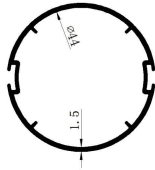
Item No.: GL1003 W: 0.69kg/m T: 1.5mm OD: \Phi 47mm ID: \Phi 44mm
